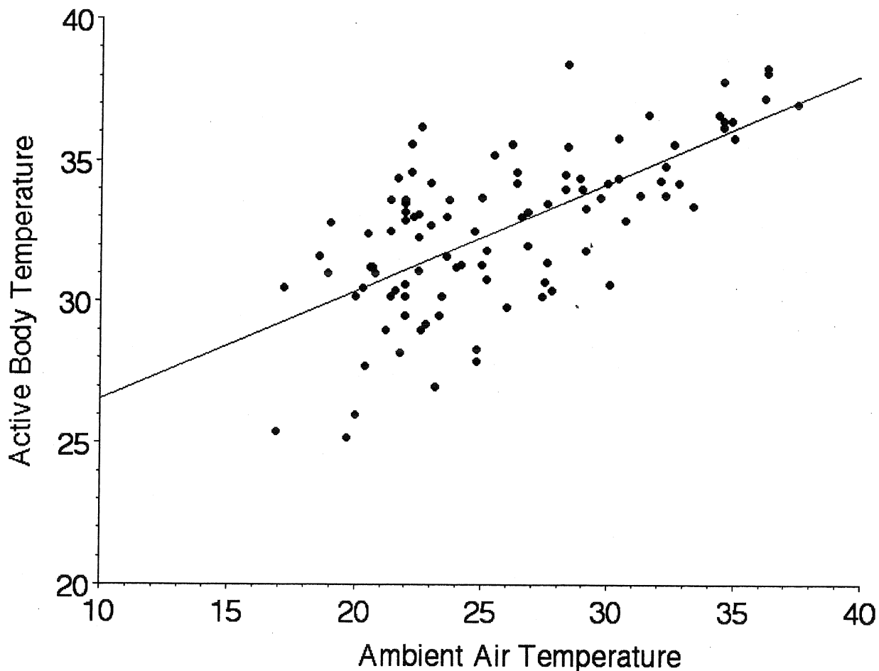
Figure 1. Active body temperature of Cryptoblepharus buehnananii plotted against ambient air temperature.
