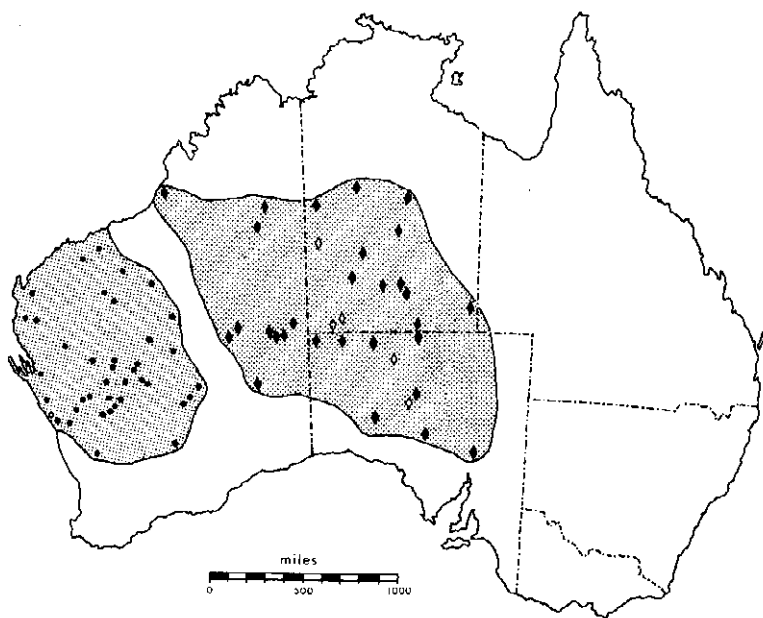
Fig. 3—The geographic distribution of Varanus caudolineatus (circles) in Western Australia, and Varanus gilleni (diamonds) in central Australia, illustrating allopatry in these lizard species. See text.
