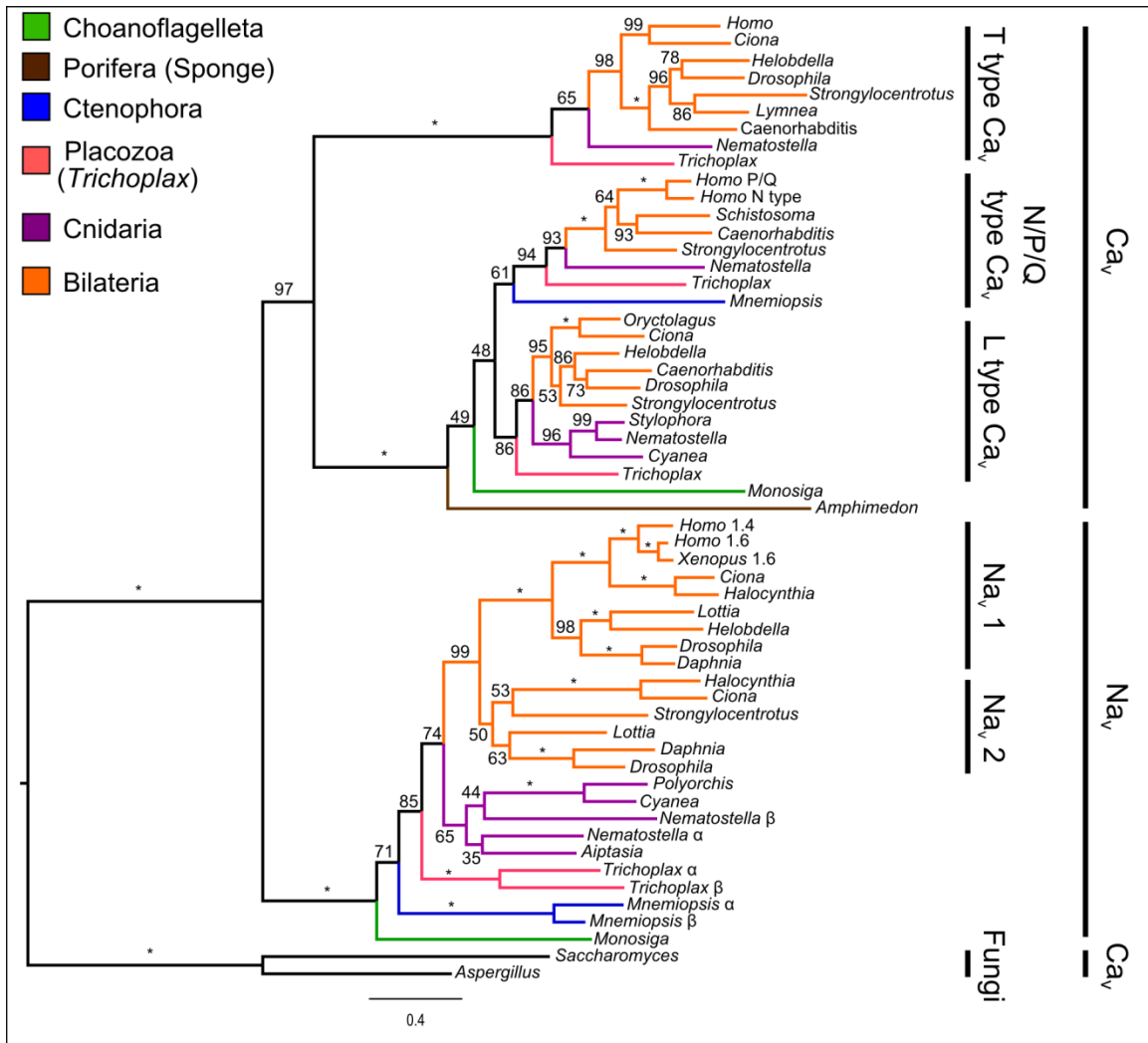
Figure 1.2: Maximum likelihood phylogeny of \text{Na}_v and \text{Ca}_v channels.
