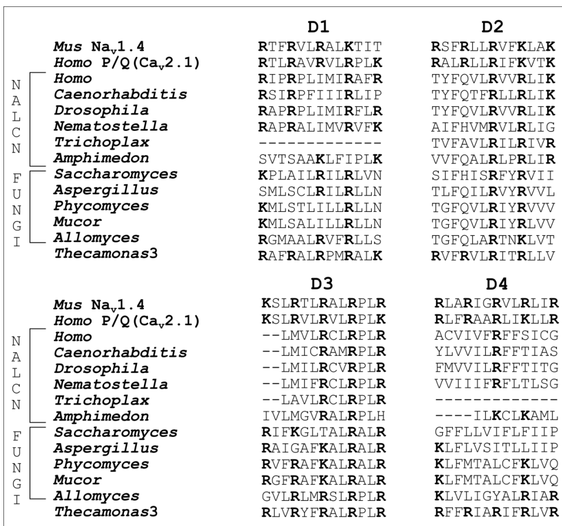
Figure 2.3: Alignment of the voltage-sensing S4 segments from four-domain ion channels.
