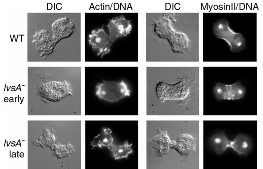
Figure 6. Actin (left) and myosin (right) distribution in wild-type (top) and lvsA mutant (middle and bottom) cells in suspension conditions. Cells were fixed in suspension and processed for actin and myosin II localization as described in Figure 5. In these conditions both wild-type and lvsA -mutant cells localize actin to their cortex and poles. Wild-type cells concentrate myosin into their cleavage furrows. However, myosin II distribution is clearly affected in the mutant cells. Early in cytokinesis (middle), myosin II begins to concentrate in the presumptive furrow, but this distribution is patchy and not as strong as that in wild-type cells. Later in cytokinesis (bottom), the distribution of myosin II is disrupted by the formation of a bulge in the middle of the cleavage furrow.
